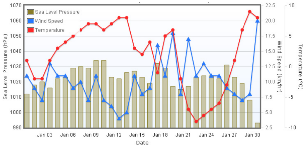
Figure B.3 Sea level pressure and temperature.
